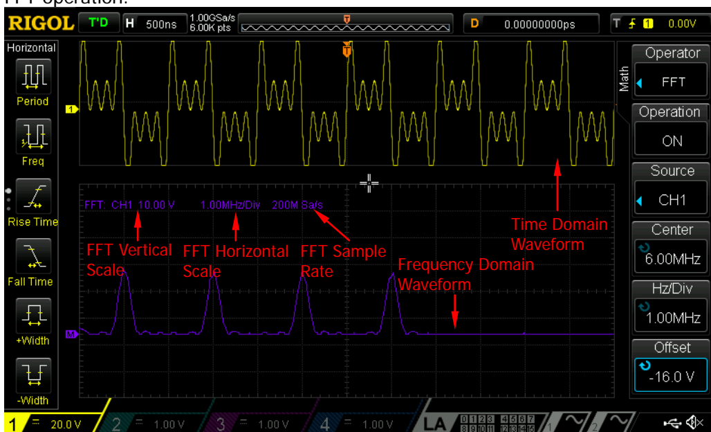
Figure 6-1 FFT Operation
