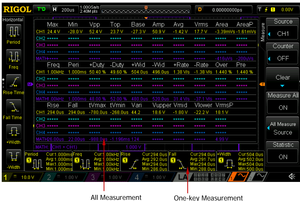
Figure 6-6 All Measurement
