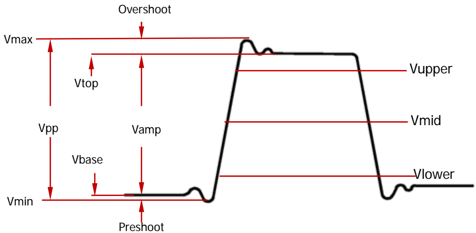
Figure 6-5 Voltage Parameters
