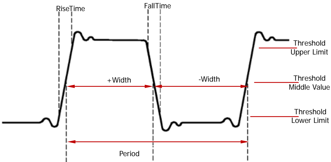
Figure 6-3 Time Parameters
